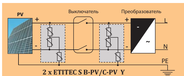
2 x ETITEC S B-PV/C-PV
